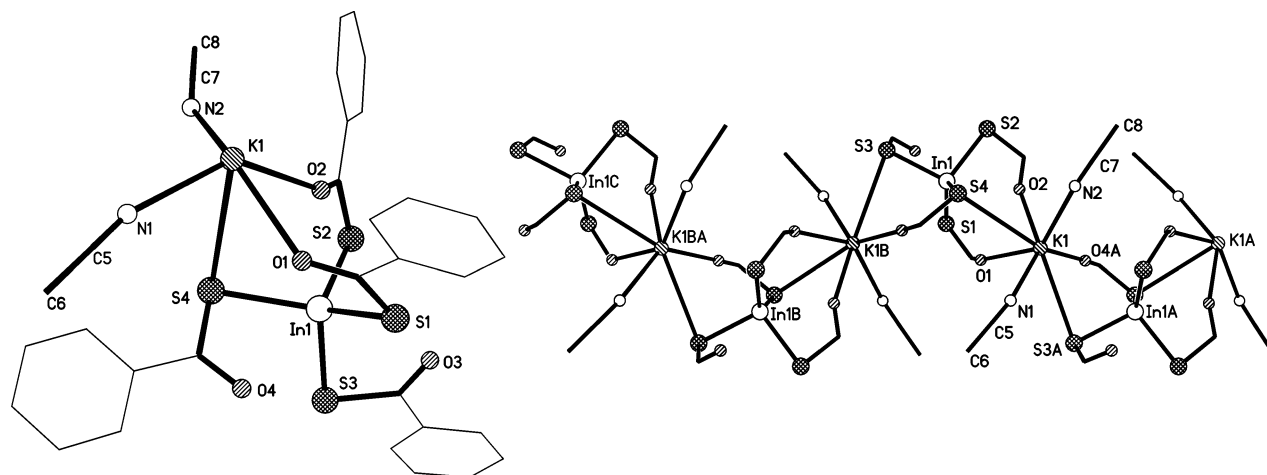
FIGURE 5. Ball and stick diagram of [KIn(SC(O)Ph)_4(MeCN)_2] and a segment of its polymeric structure.
