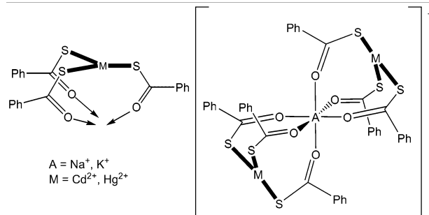
Scheme 3. Views of the 'Claw-like' [\text{M}(\text{SC}\{\text{O}\}\text{Ph})_3]^- Ions ( \text{M} = \text{Zn}, \text{Cd}, and \text{Hg} ) and Its Complex with Alkali-Metal Ions
